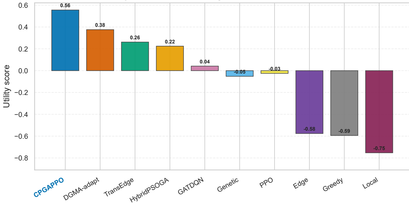
UtilityScore (cross-DAG avg, mean \pm 95% CI over seeds)
